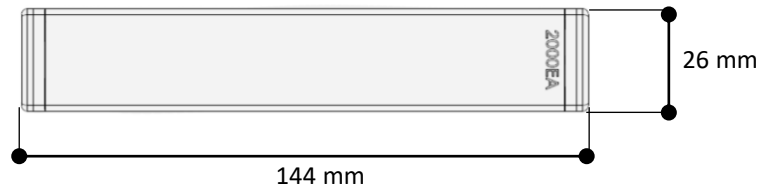
2000 Modular Vent
